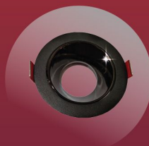
FIXTURE & ACCESSORIES INF046-B FIXTURE for Modul / MR16 > Black Ring > Pearl Black Cup > Body Size : 85x1130mm > Cut Size : 75mm
