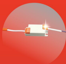
DRIVER INDR020-4 TUNEABLE CCT > 5,5w-7,5w 250ma > Input : 170v-240v > Output : 12v-21v 250ma > Frequency Range : 50-60Hz
